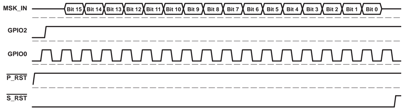
Figure 3–3. Clock Mask Read Timing After Reset
